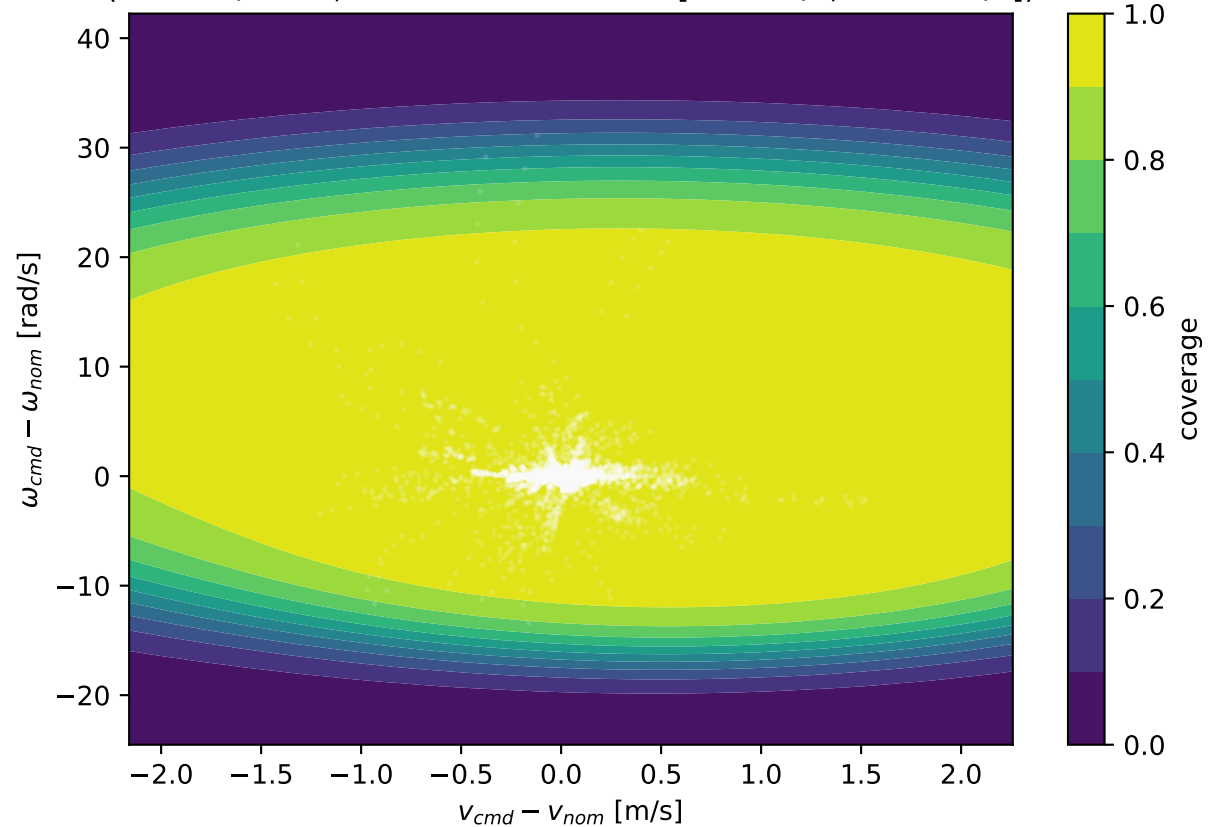
Residual coverage vs command offset (0 = off / OOD; state fixed at mean [0.34 m/s, 0.05 rad/s])
